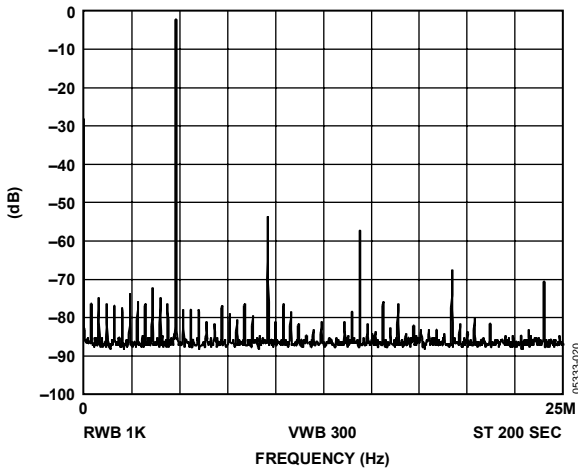
Figure 28. f_{MCLK} = 50 MHz; f_{OUT} = 4.8 MHz, Frequency Word = 189374C
