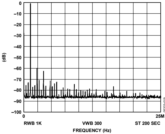
Figure 27. f_{MCLK} = 50 MHz; f_{OUT} = 1.2 MHz, Frequency Word = 0624DD3
