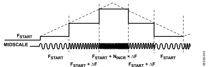
Figure 32. Triangular-Sweep Profile
