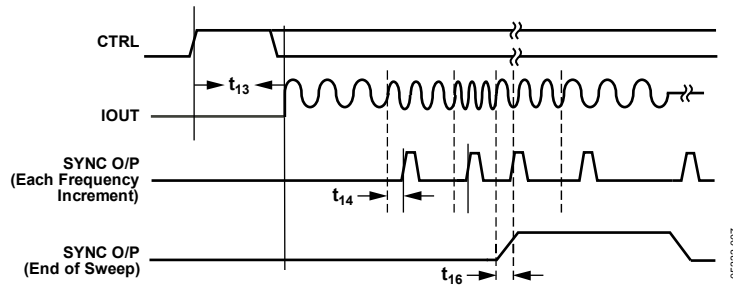
Figure 7. CTRL Timing, Triangular-Sweep Mode
