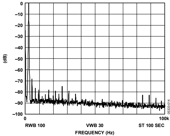
Figure 22. f_{MCLK} = 10 \text{ MHz} ; f_{OUT} = 2.4 \text{ kHz} , Frequency Word = 000FBA9
