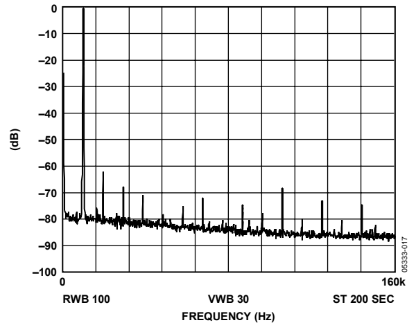
Figure 25. f_{MCLK} = 50 \text{ MHz} ; f_{OUT} = 12 \text{ kHz} , Frequency Word = 000FBA9
