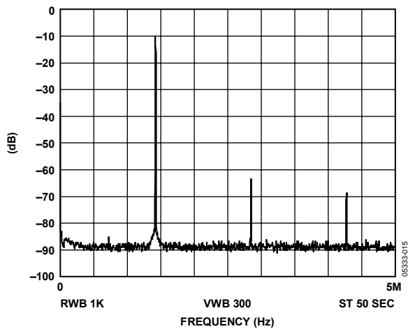
Figure 23. f_{MCLK} = 10 \text{ MHz} ; f_{OUT} = 1.43 \text{ MHz} = f_{MCLK}/7 , Frequency Word = 2492492
