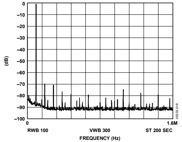
Figure 26. f_{MCLK} = 50 \text{ MHz} ; f_{OUT} = 120 \text{ kHz} , Frequency Word = 009D496
