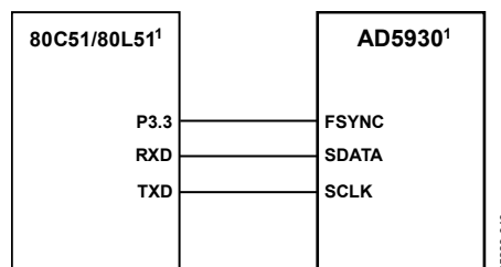
ADDITIONAL PINS OMITTED FOR CLARITY.
