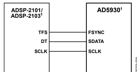
Figure 36. ADSP-2101/ADSP-2103 to AD5930 Interface
