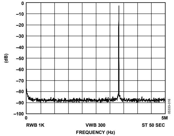
Figure 24. f_{MCLK} = 10 \text{ MHz} ; f_{OUT} = 3.33 \text{ MHz} = f_{MCLK}/3 , Frequency Word = 5555555
